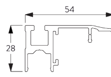
SG 8643 Side guide case inside fitting
