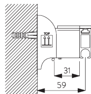
For parallel fixing of profile to the wall
